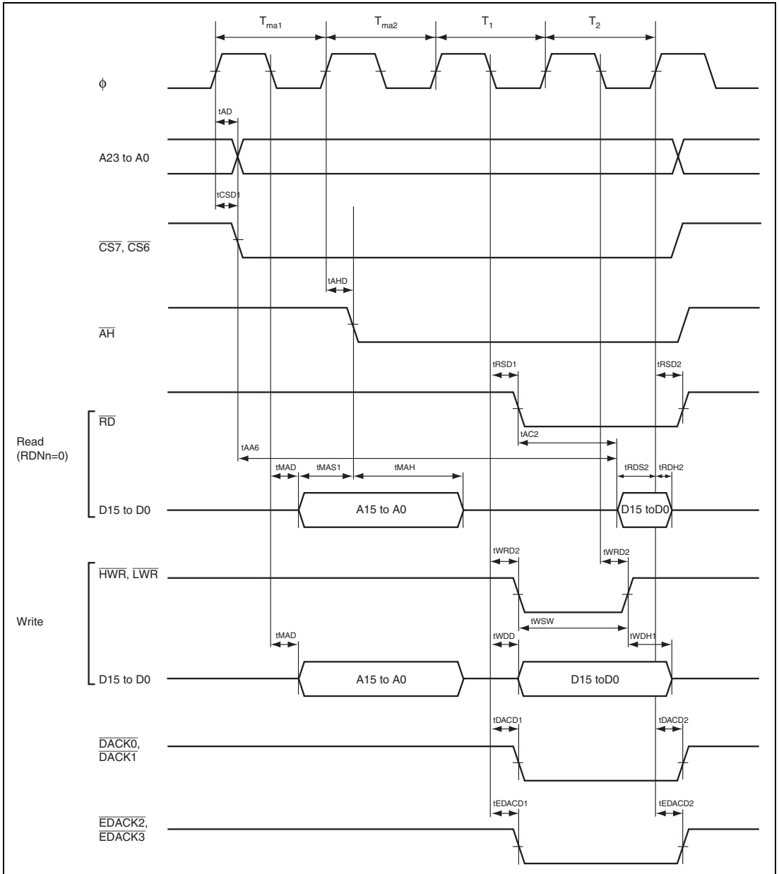
Figure 26.34 Multiplexed Bus Timing: Data Two-State Access
