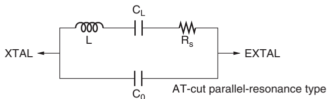
Figure 23.3 Crystal Resonator Equivalent Circuit
