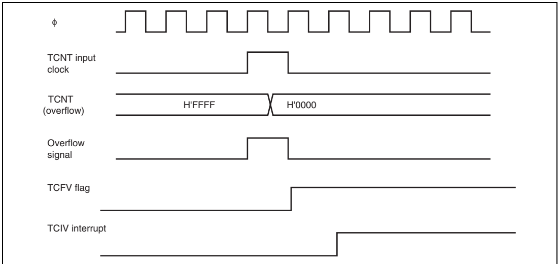
Figure 11.41 TCIV Interrupt Setting Timing
