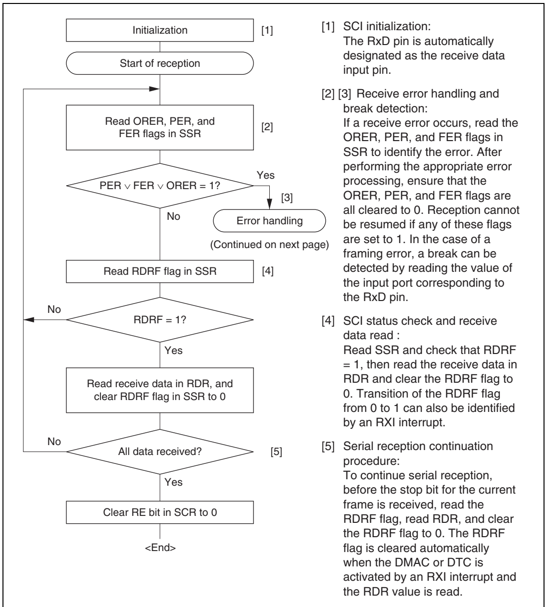
Figure 15.9 Sample Serial Reception Data Flowchart (1)
