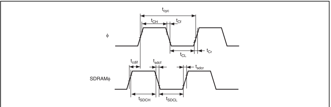
Figure 26.4 SDRAM \phi Timing
