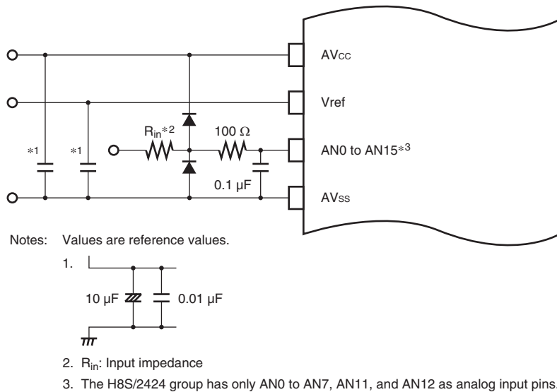
Figure 17.12 Example of Analog Input Protection Circuit
