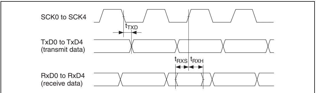
Figure 26.45 SCI Input/Output Timing: Synchronous Mode
