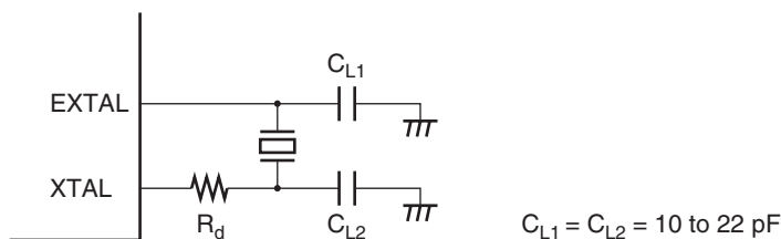
Figure 23.2 Connection of Crystal Resonator (Example)
