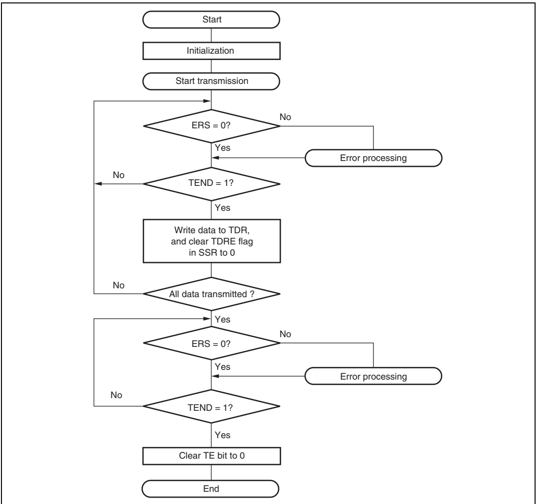
Figure 15.28 Example of Transmission Processing Flow
