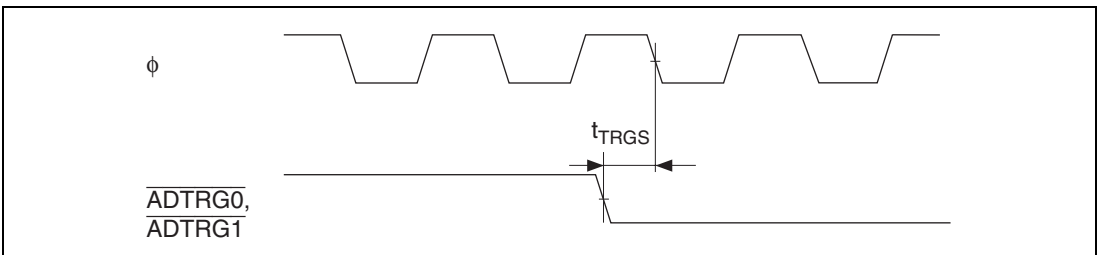
Figure 26.46 A/D Converter External Trigger Input Timing
