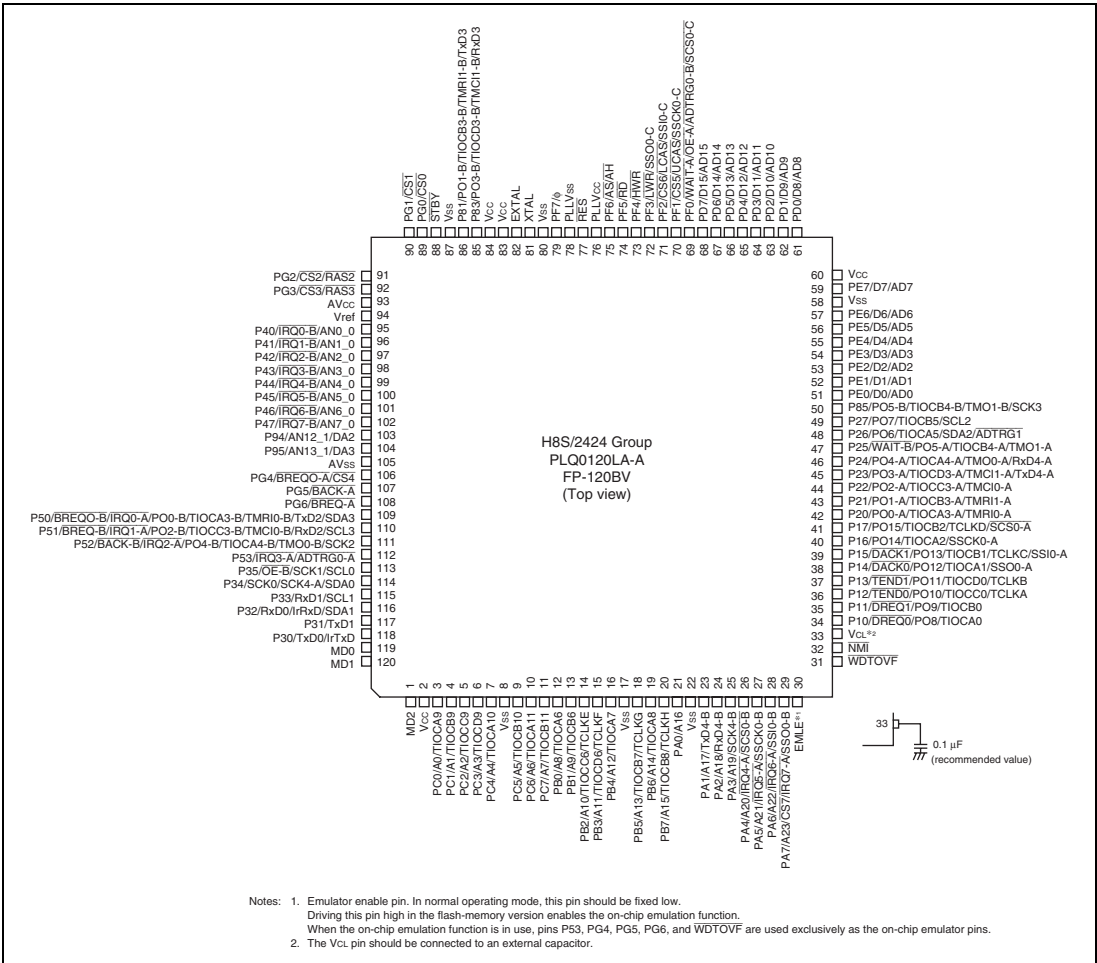
Figure 1.6 Pin Assignments for H8S/2424 Group
