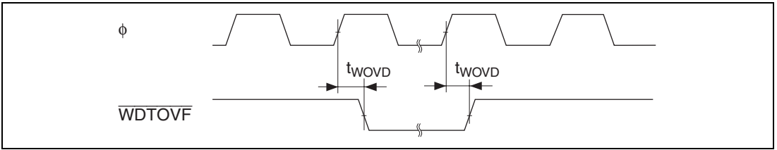
Figure 26.43 WDT Output Timing
