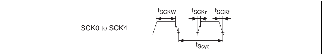
Figure 26.44 SCK Clock Input Timing
