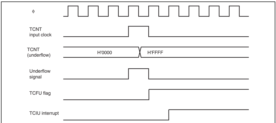
Figure 11.42 TCIU Interrupt Setting Timing
