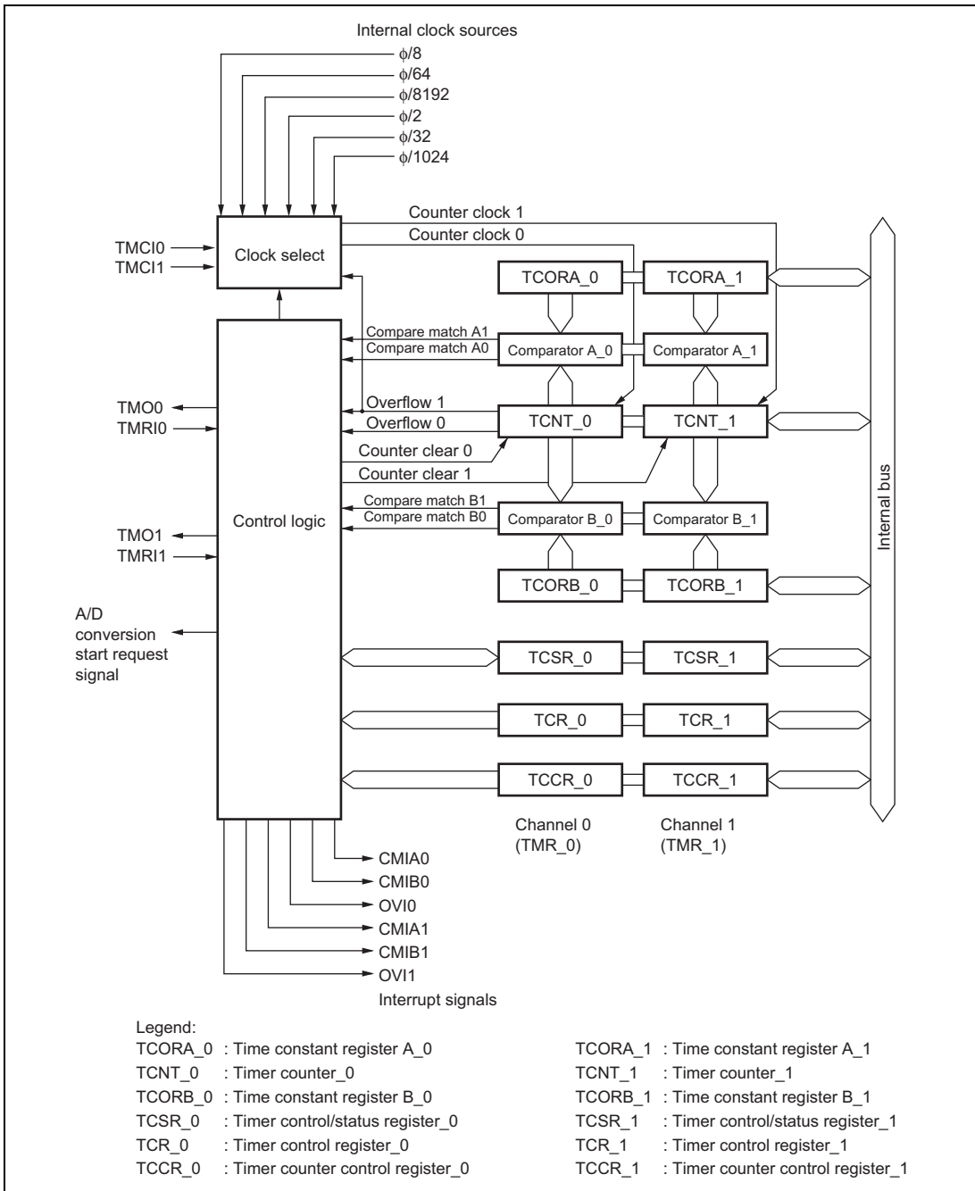
Figure 13.1 Block Diagram of 8-Bit Timer Module
